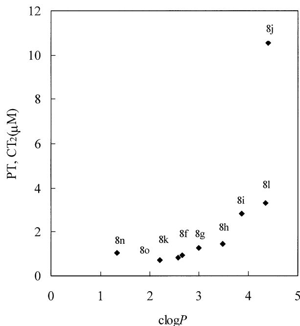
Figure 3. The correlation between \log P and CT_2 (PT) of sulfonamide derivatives. \log P was calculated using TSAR ver. 3.0 (Oxford Molecular Group). PT, CT_2 ; see corresponding footnotes b and c in Table 3.
